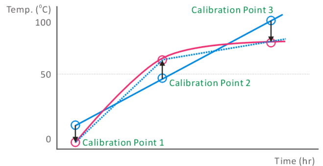
— Chamber Temperature Profile — Controller Temperature Profile ..... 3 Point Calibrated Temperature Profile
