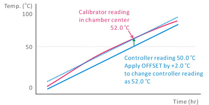
— Chamber Temperature Profile — Controller Temperature Profile ..... 1 Point OFFSET Temperature Profile
